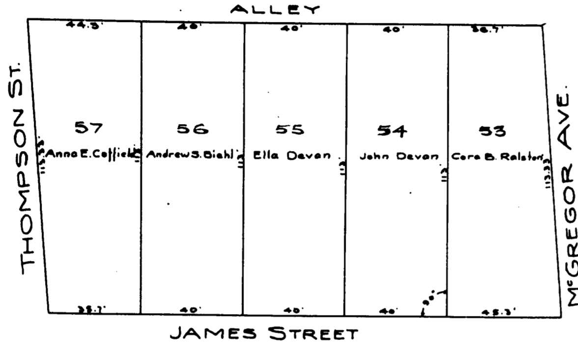
RALSTON ET AL. ALTERATION OF MCGREGOR'S 2 ND ADDITION TO SHADYSIDE BELMONT CO., OHIO. Scale 1"=33' Aug 15, 1910
